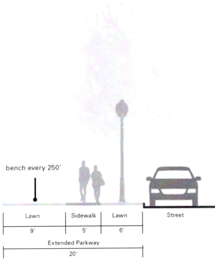
Extended Parkway Section on Future Public-Public Open Space
