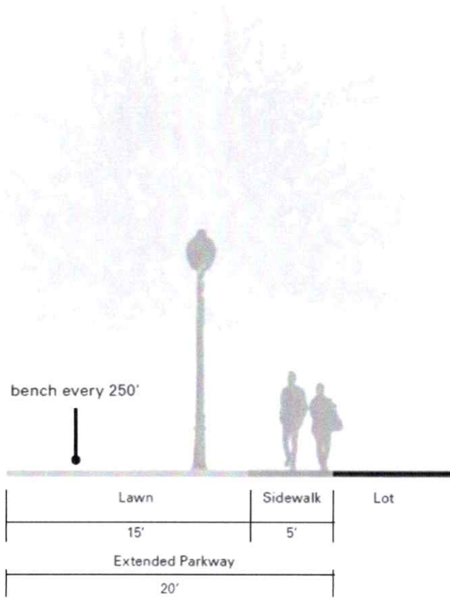
Extended Parkway Section on Future Public-Public Open Space
